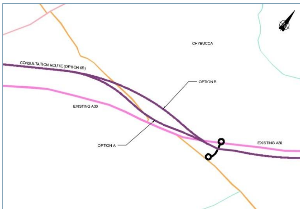
Figure 7-4: Chybucca - public consultation layout
